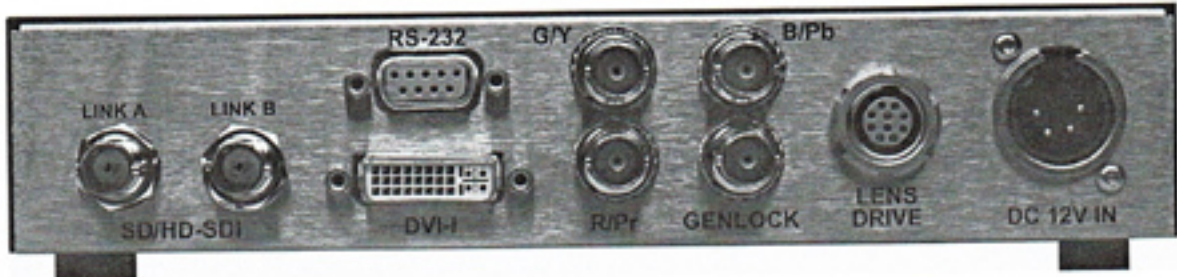
Figure 3. CCU connectors – rear panel
