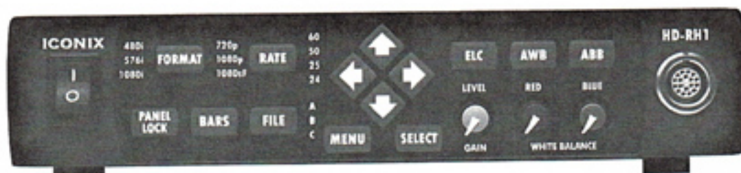
Figure 2. CCU – front panel
